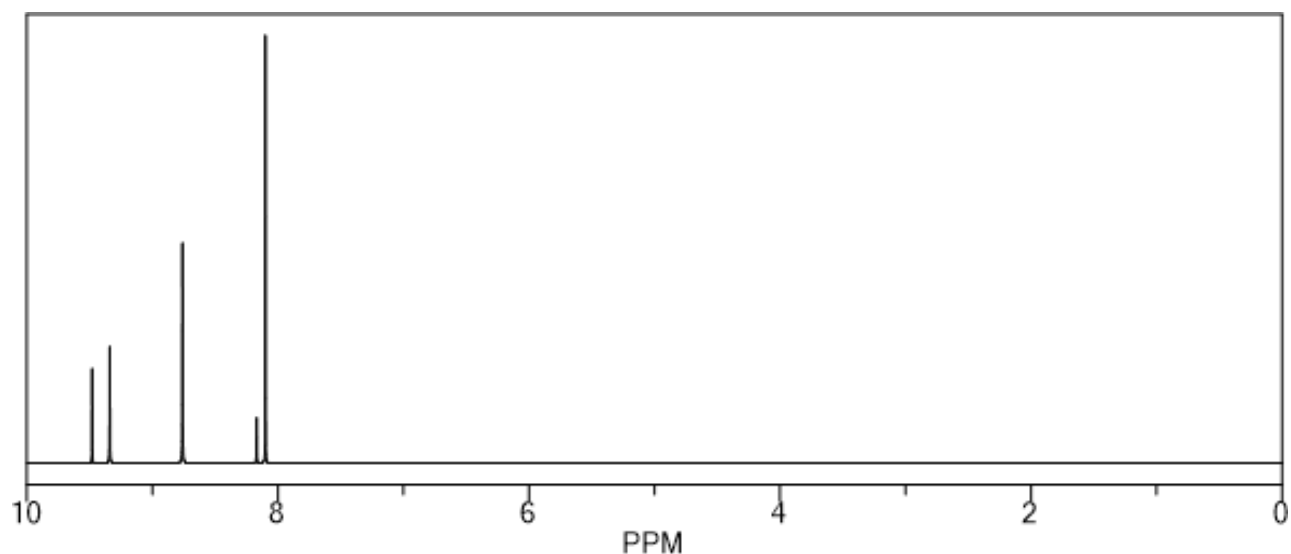
Figure 5. ^1\text{H} NMR spectrum of N,N' -(1,4-phenylenebis(methanylylidene))bis(pyrazine-2-carboxamide)
