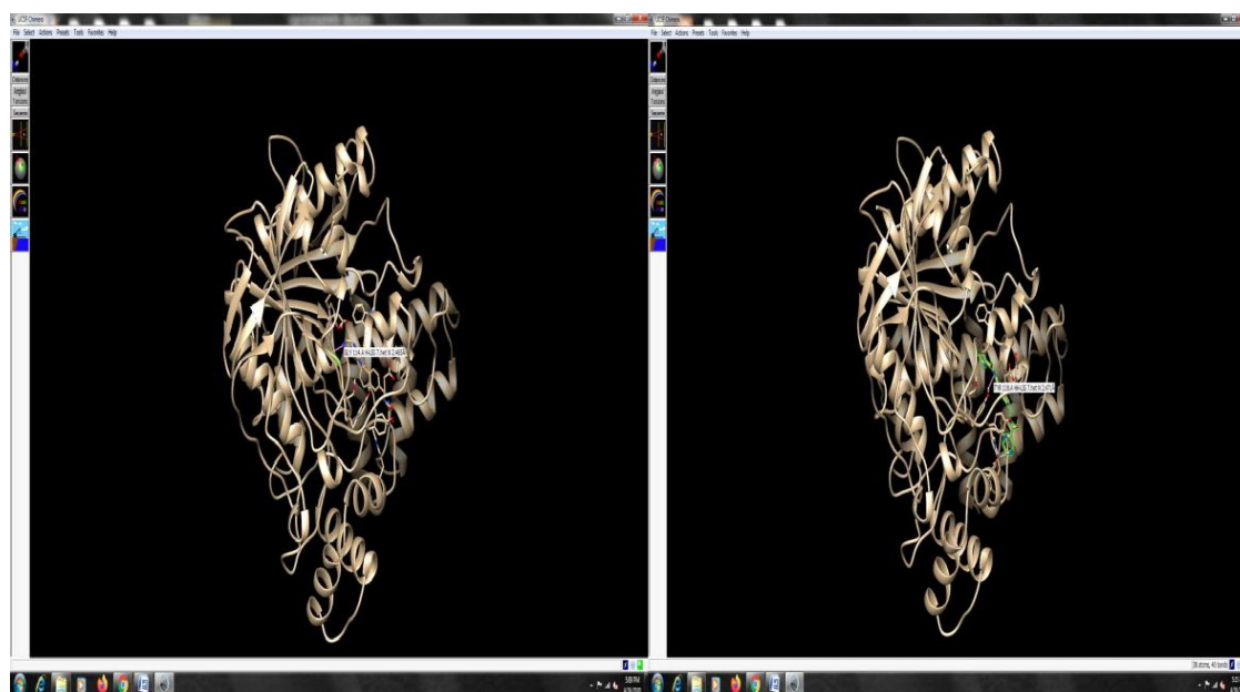
Plate 4. Docking interaction of ligand and receptor using autodock
