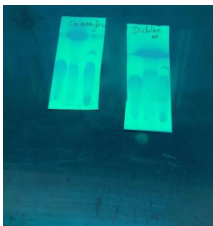
Plate.3 TLC Plate for(Teraphthaldehyde) pyrazinamide
