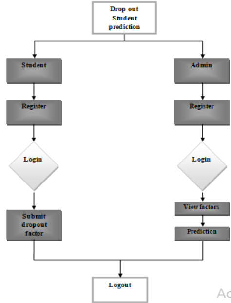
Fig Data Flow diagram
